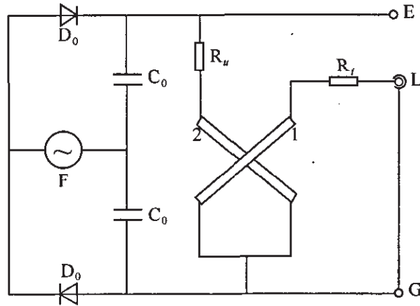
绝缘电阻表原理图
